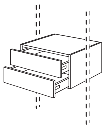
U2SBL-36 DRAWER UNIT 2 drawers, includes unit connectors widths: 300, 400, 450, 500, 600, 800, 900 mm
