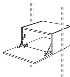
UKBBL-36 BASE UNIT WITH BAR FLAP 1 flap with opening support mechanism, includes unit connectors widths: 450, 500, 600, 800, 900 mm
