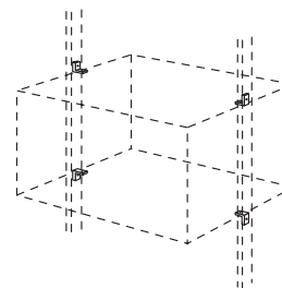
ABLS15-02 / ABL530-02 UNIT CONNECTOR 4 pieces including screws and sliding block as set, for mounting wall units on Backlight support poles Available colours: No. 073 Stainless steel finish No. 010 Black
