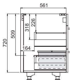
WASTE SEPARATION SYSTEM SEPARATO, 600 MM WIDE
